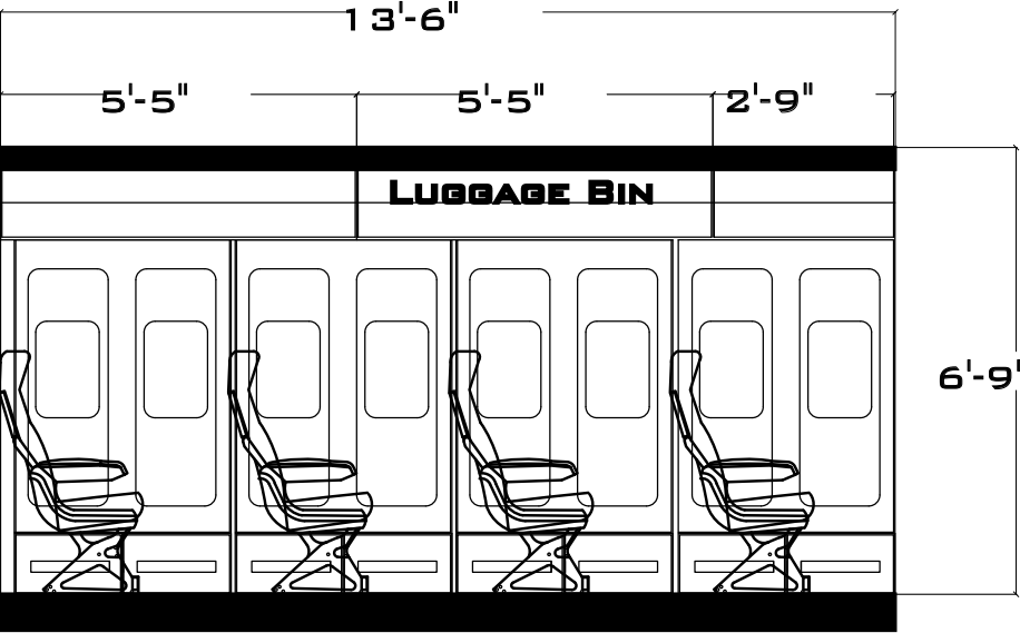
ECONOMY SEATS SECTIONAL VIEW
