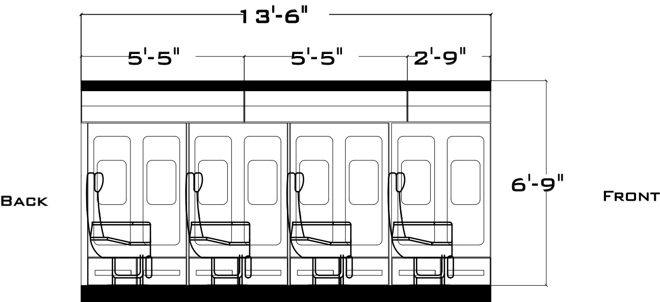
EXECUTIVE SEATS SECTIONAL VIEW
