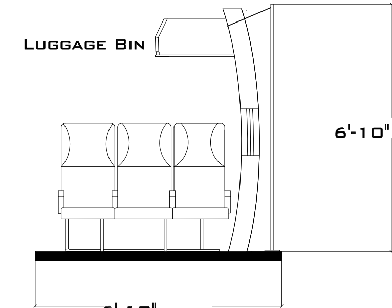
FRONT ECONOMY SEATS SECTIONAL VIEW
